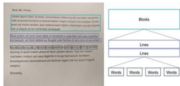
Figure 2 - Text structure
